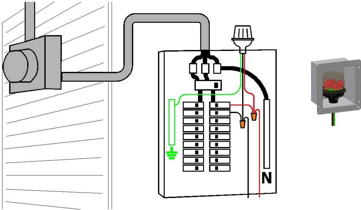
Pigtailling into existing branch circuits
