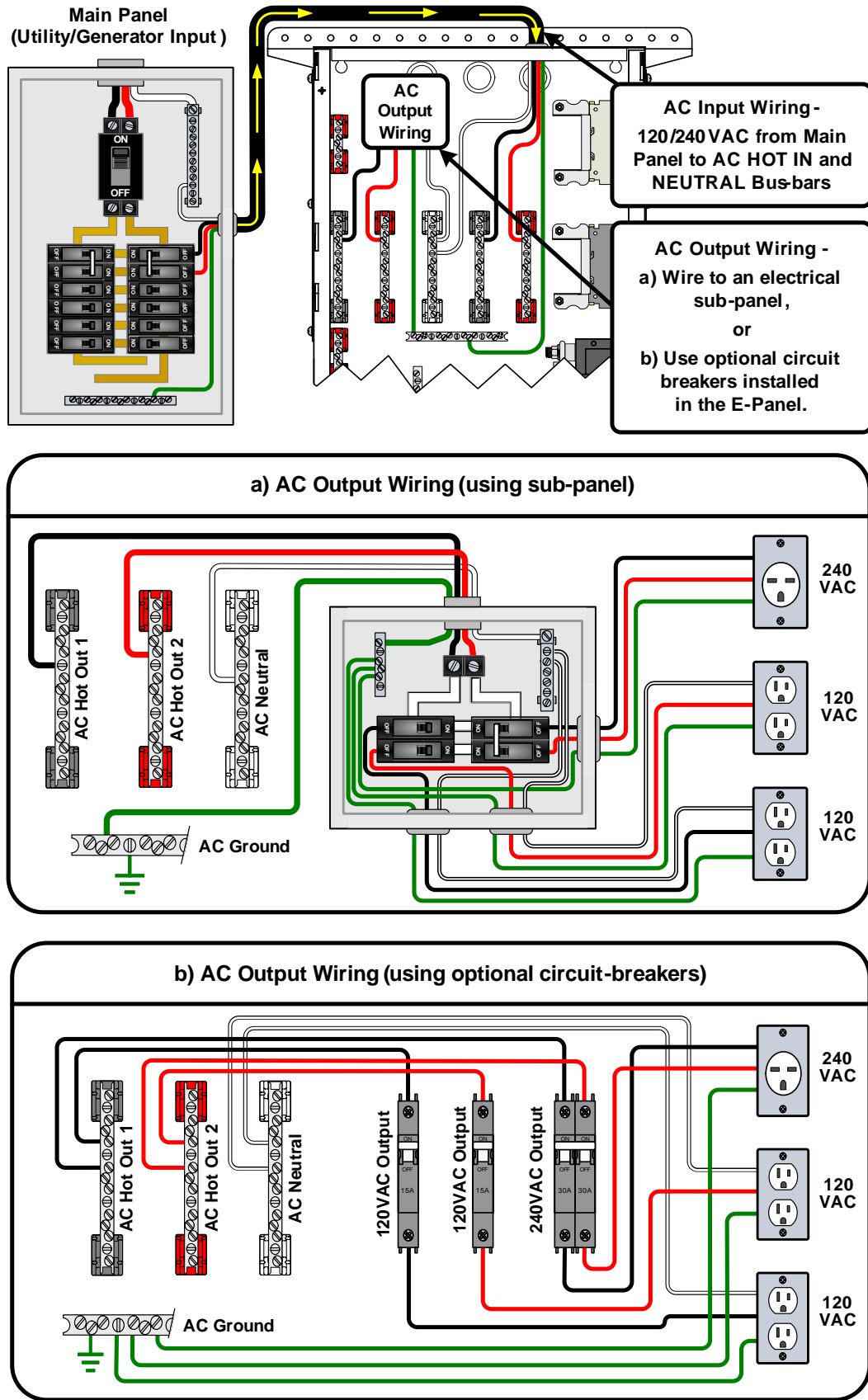
Figure 14, E-Panel AC Input and Output Wiring
