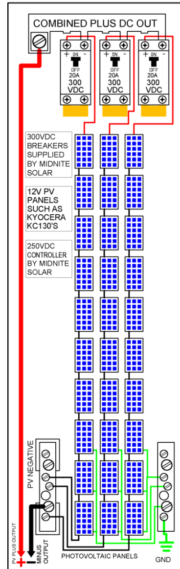
DIAGRAM USING TEN 12 VOLT PANELS IN SERIES INTENDED TO FEED A 250 VOLT MPPT CHARGE CONTROLLER. THIS SYSTEM HAS 3900 WATTS OF PV.
